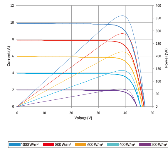
Current- Voltage & Power- Voltage Curve (365S)
